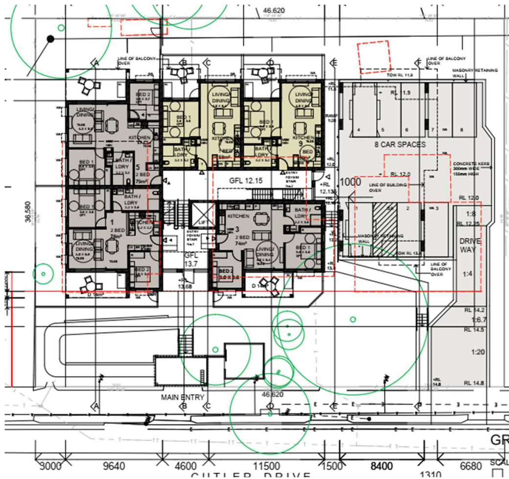
Figure 2 – Ground Floor Plan extract showing the proposed layout of the development Source: Barry Rush & Associates November 2022
